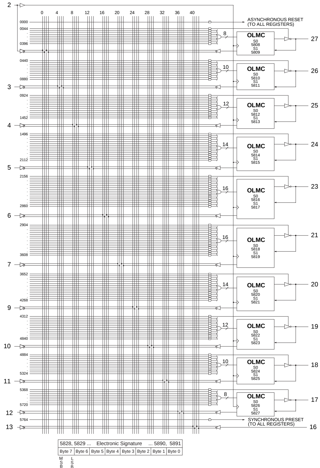
PLCC & SSOP Package Pinout
