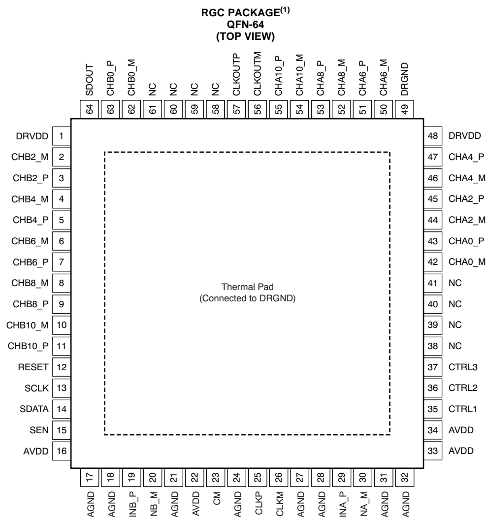
Figure 2. ADS58C28 LVDS Pinout
