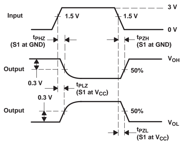
VOLTAGE WAVEFORMS
