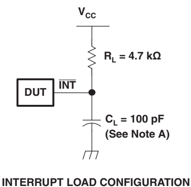
INTERRUPT LOAD CONFIGURATION
