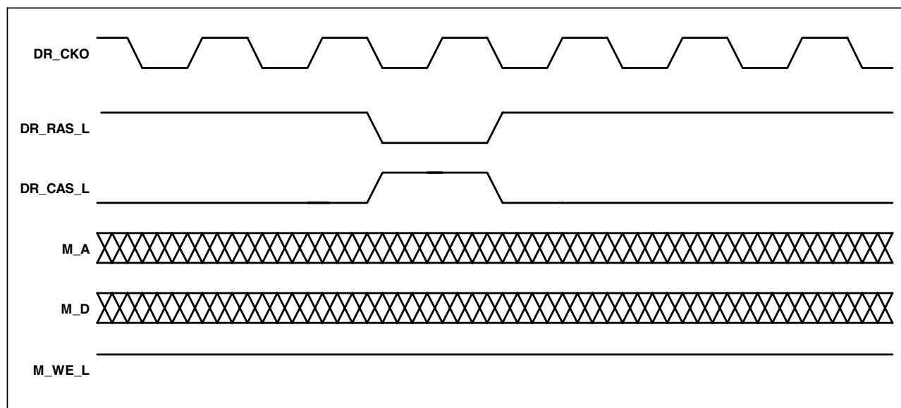
Figure 5. SDRAM Refresh
