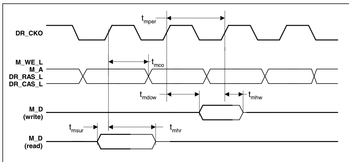
Figure 1. SDRAM Timing
