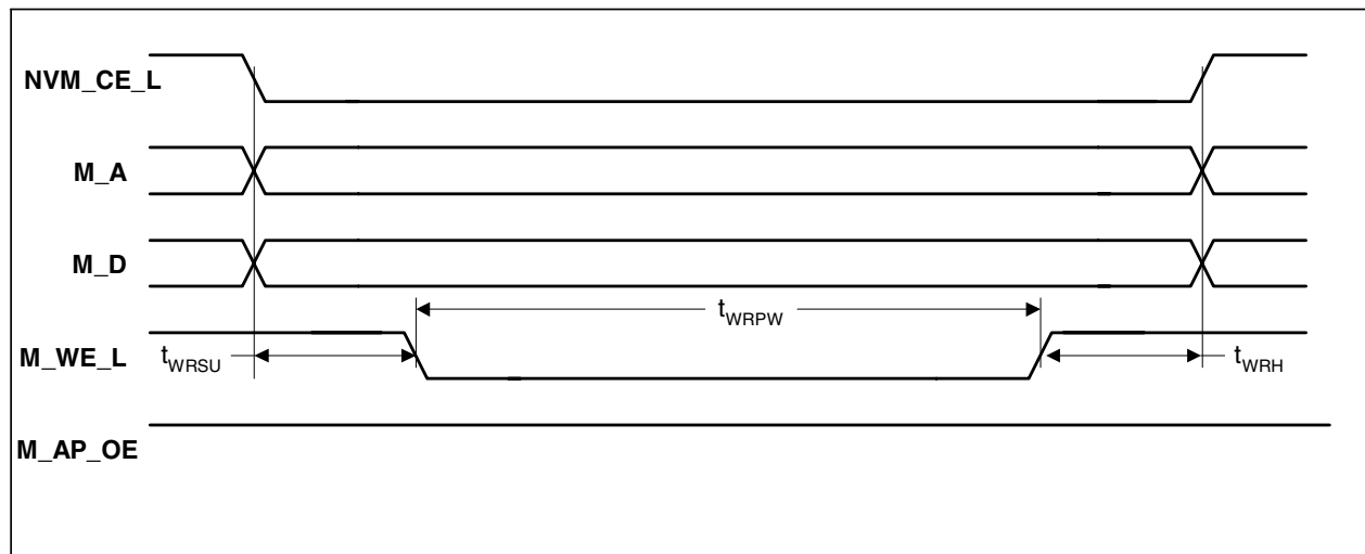
Figure 11. FLASH/ROM Write
