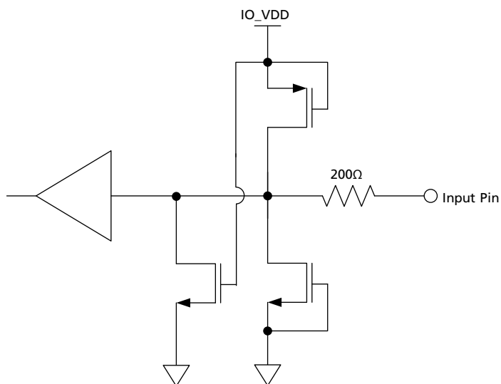
Figure 3-4: Digital Input Pin with weak pull-down - maximum pull-down current <110mA (JTAG/ \overline{\text{HST}} , STANDBY, SCLK_TCK, SDIN_TDI, TCK, TDI)
