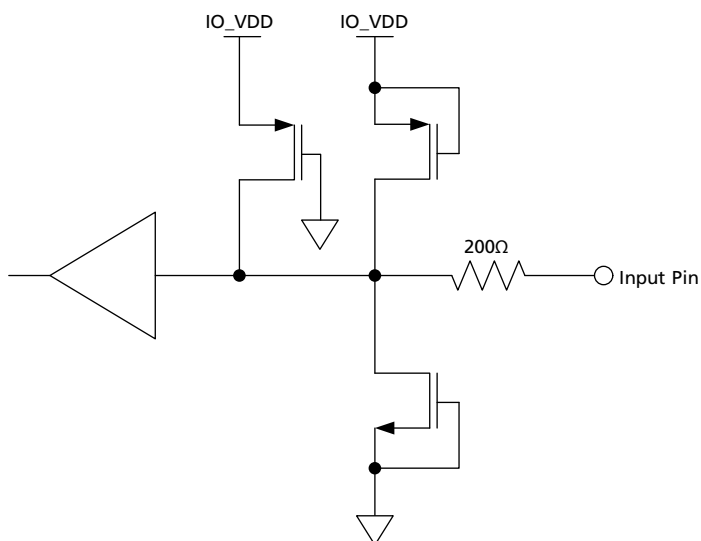
Figure 3-5: Digital Input Pin with weak pull-up - maximum pull-up current <110mA ( \overline{CS\_TMS} , SDO\_EN/\overline{DIS} , TMS )
