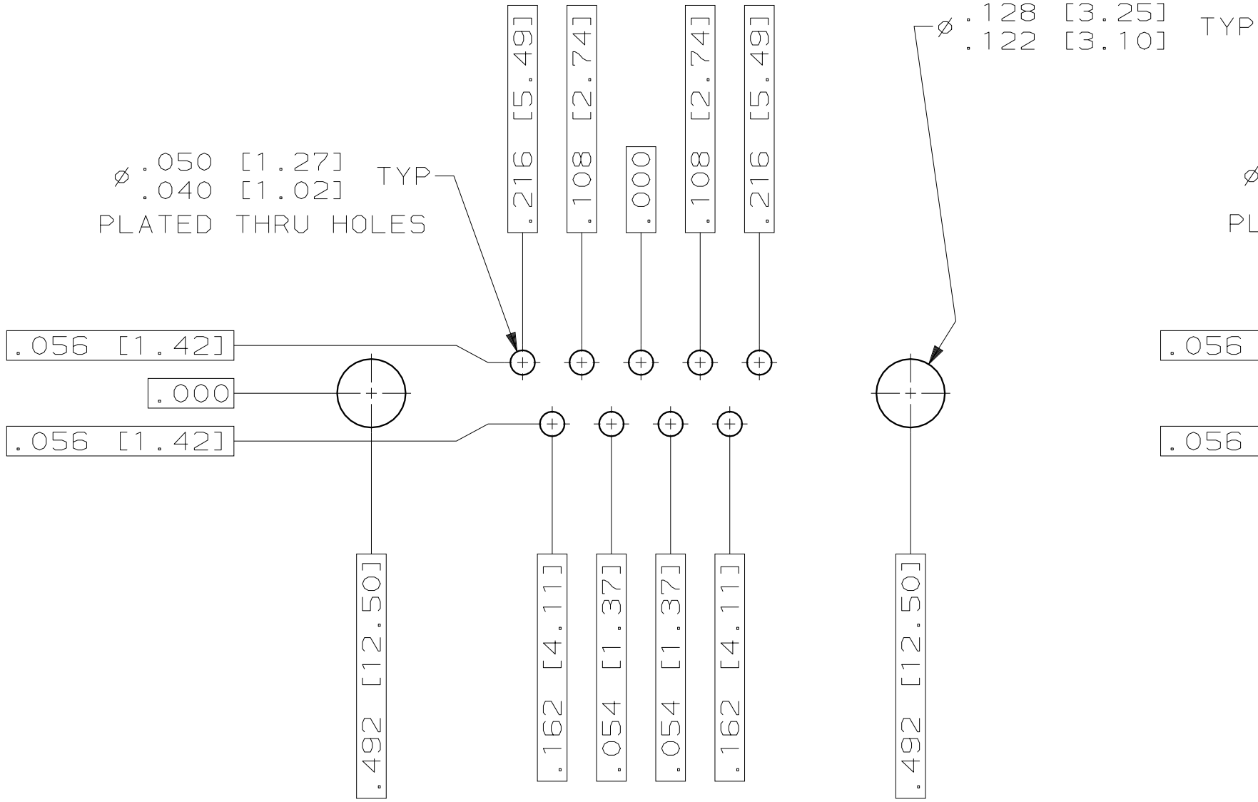
RECOMMENDED P.C. BOARD LAYOUT SHELL SIZE 1 (9 POSITION)
