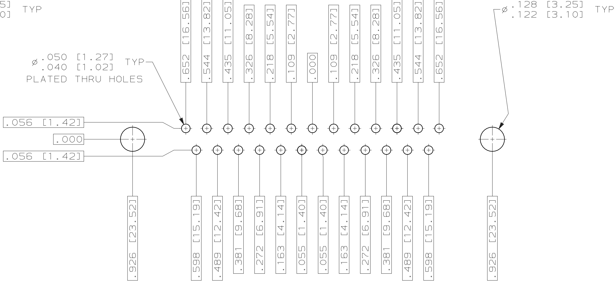
RECOMMENDED P.C. BOARD LAYOUT SHELL SIZE 3 (25 POSITION)
