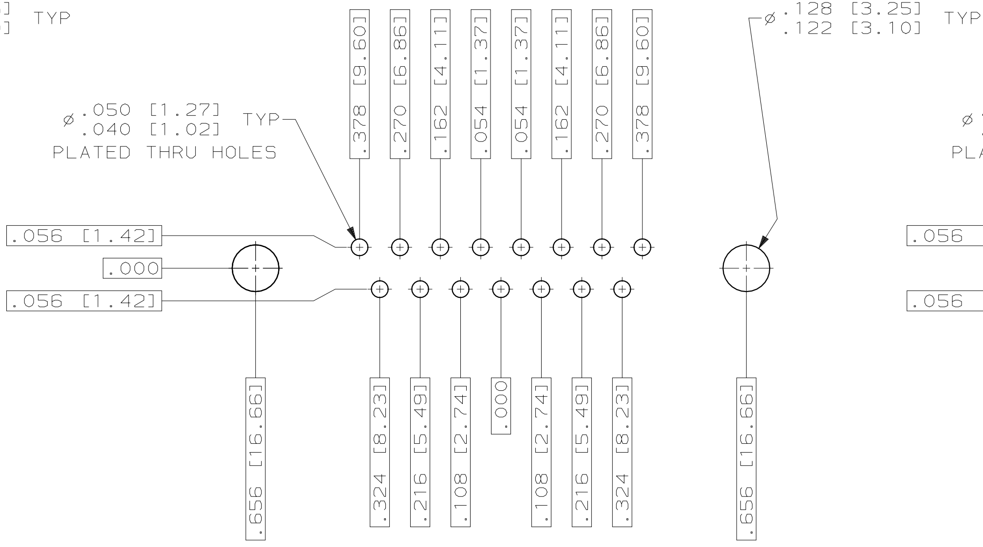
RECOMMENDED P.C. BOARD LAYOUT SHELL SIZE 2 (15 POSITION)
