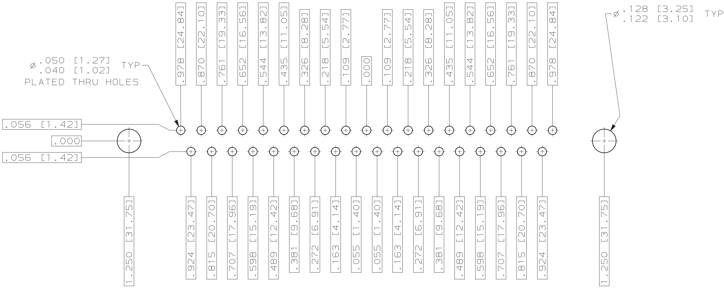
RECOMMENDED P.C. BOARD LAYOUT SHELL SIZE 4 (37 POSITION)
