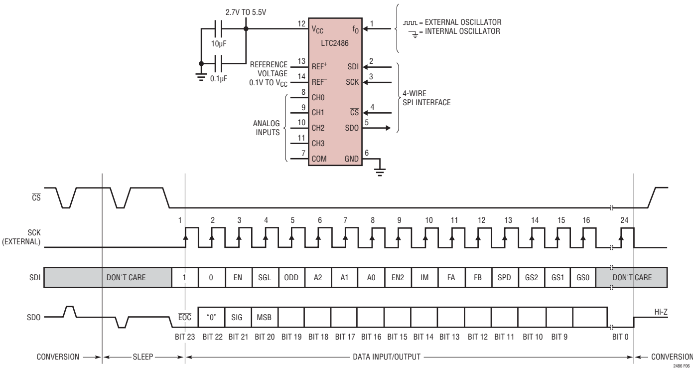
Figure 6. External Serial Clock, Single Cycle Operation
