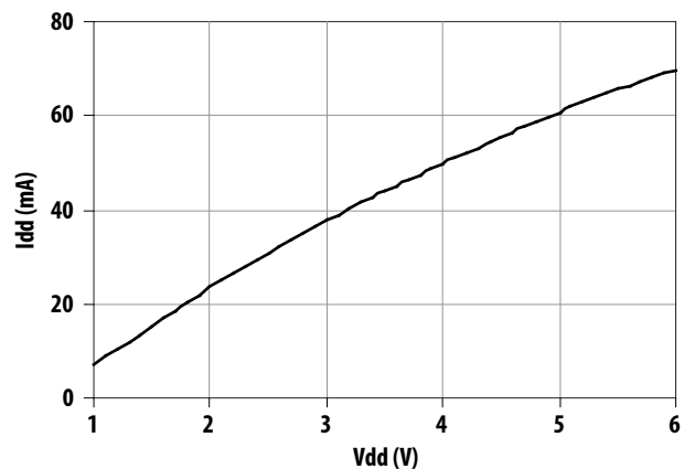
Figure 8. Total Current [1]
