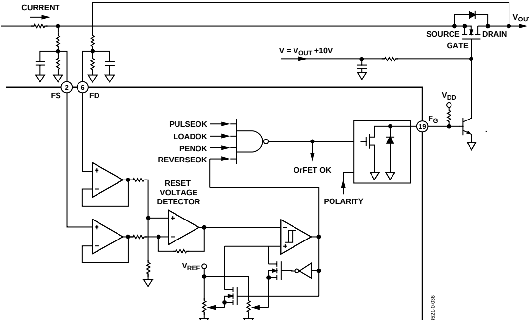
Figure 21. OrFET Gate Drive Circuit
