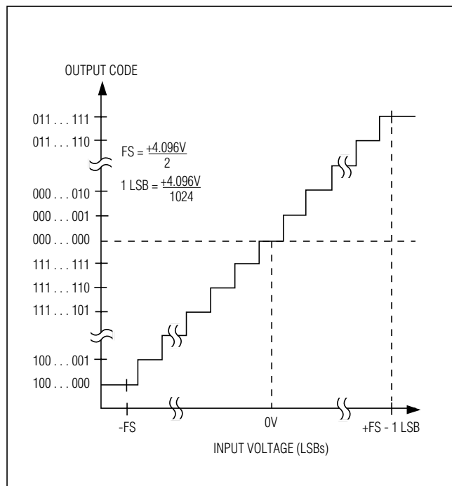
Figure 16. Bipolar Transfer Function, \pm 4.096V/2 = \text{Full Scale}
