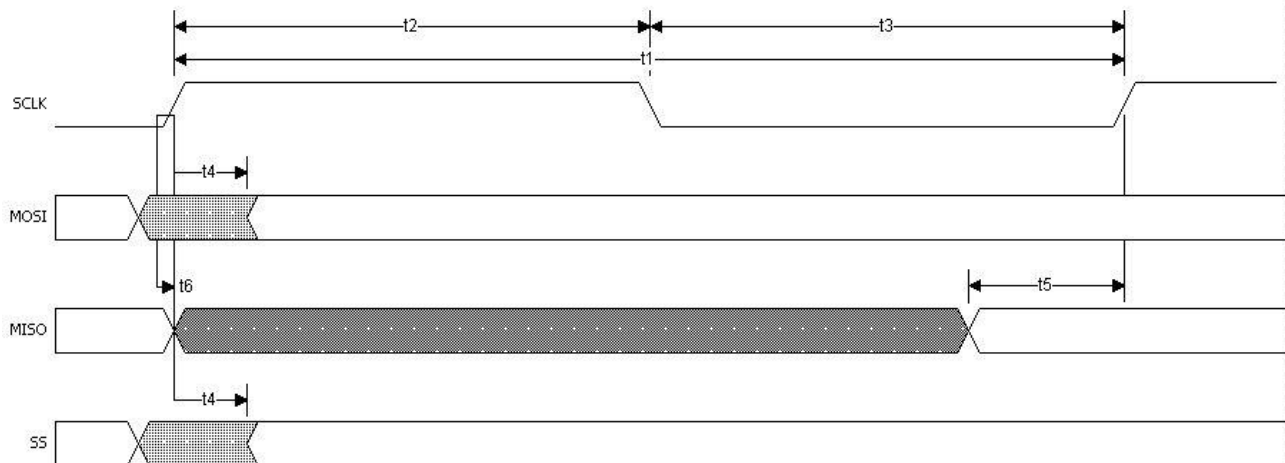
Figure 6.21 Typical SPI Master Timing
