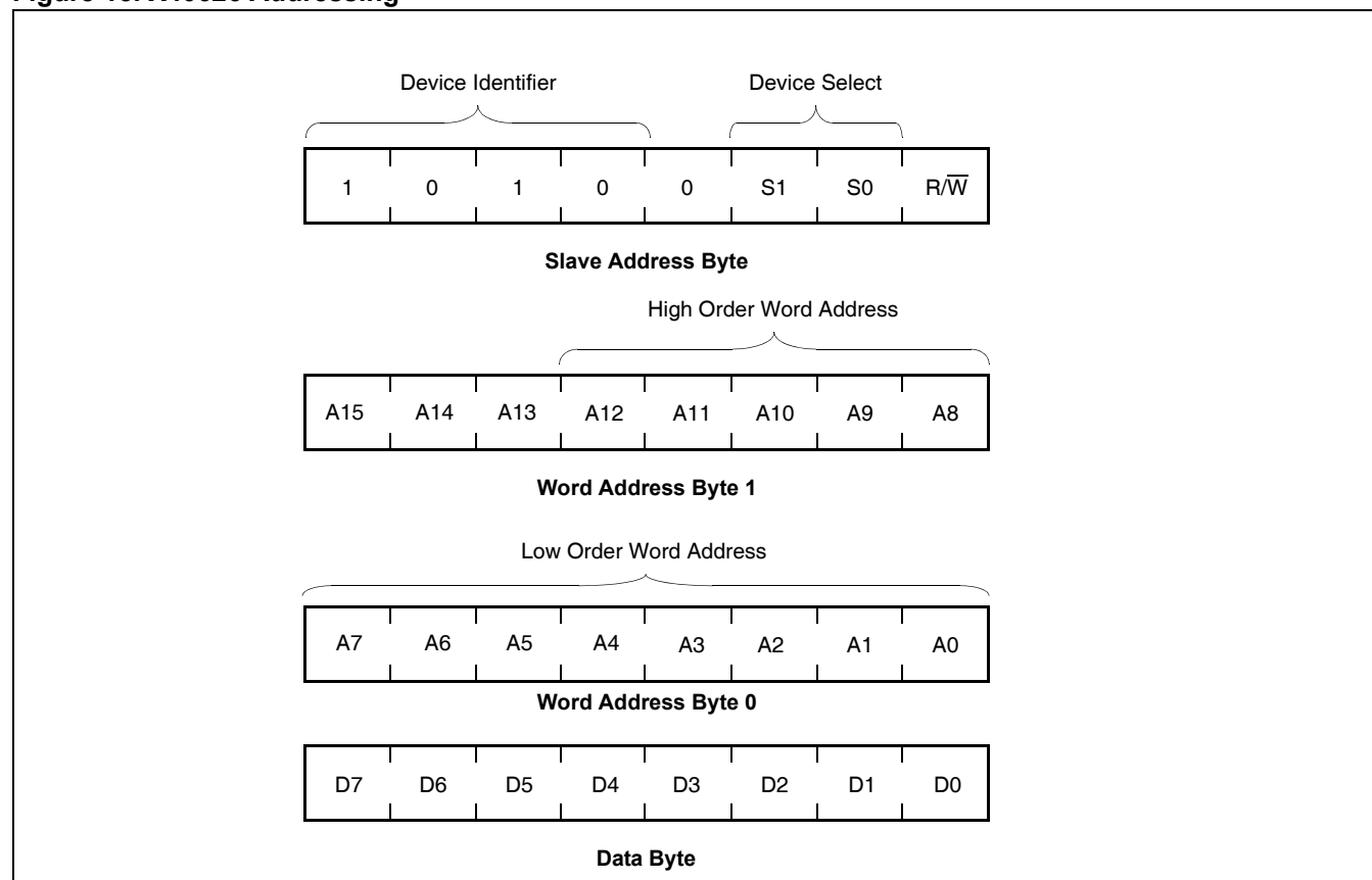
Figure 15. X40626 Addressing
