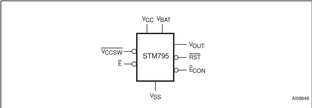
Figure 3. Logic diagram (STM795)
