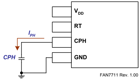
Figure 30. Preheating Timer
