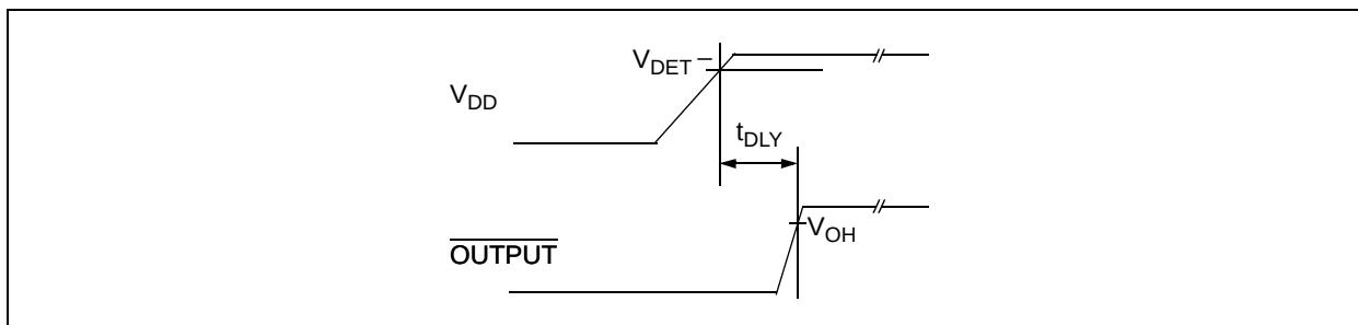
FIGURE 1-1: Timing Diagram.
