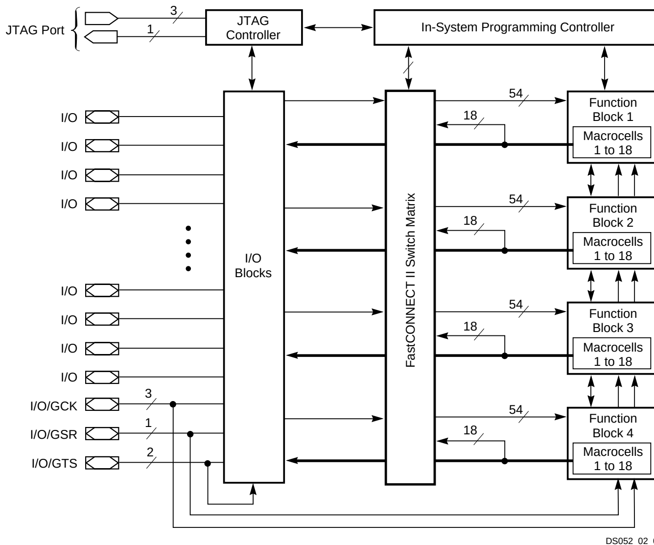
Figure 2: XC9572XV Architecture
