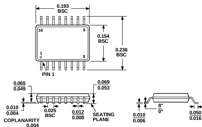
Figure 70. 16-Lead Shrink Small Outline Package [QSOP] (RQ-16) Dimensions in Inches
