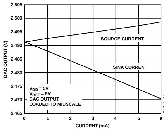
Figure 20. DAC V_{OUT} Source and Sink Current Capability
