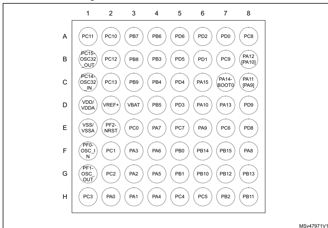
Figure 10. STM32G071Rxl UFBGA64 ballout
