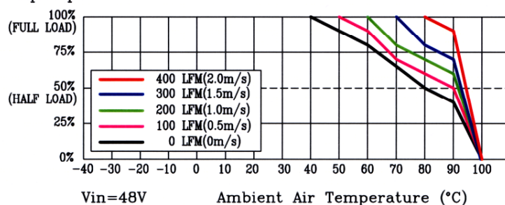
output power
