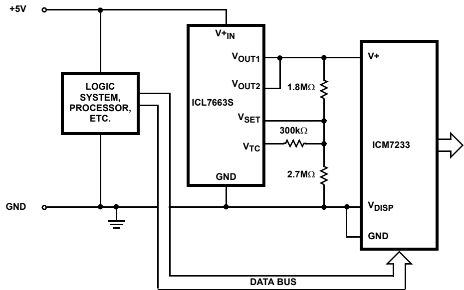
FIGURE 11. GENERATING A MULTIPLEXED LCD DISPLAY DRIVE VOLTAGE
