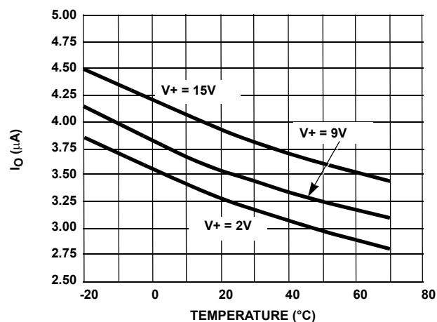
FIGURE 6. QUIESCENT CURRENT AS A FUNCTION OF TEMPERATURE
