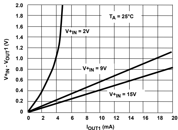
FIGURE 2. V_{OUT1} INPUT-OUTPUT DIFFERENTIAL vs OUTPUT CURRENT
