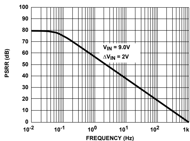
FIGURE 4. NPUT POWER SUPPLY REJECTION RATIO
