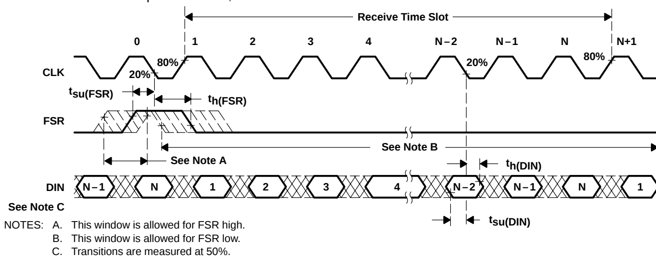
Figure 1. Fixed-Data Rate Mode, Receive Side Timing Diagram
