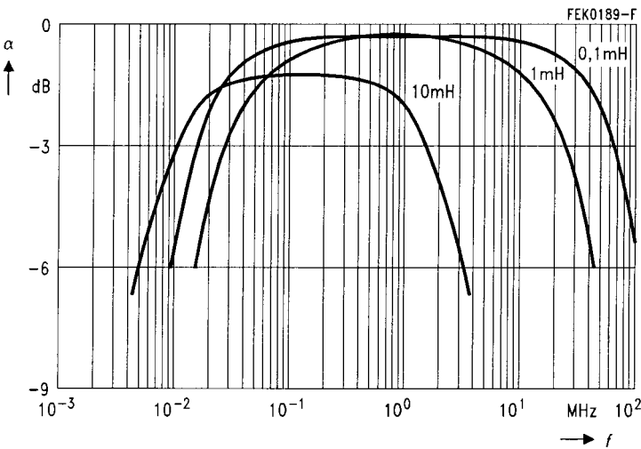
Attenuation versus frequency
