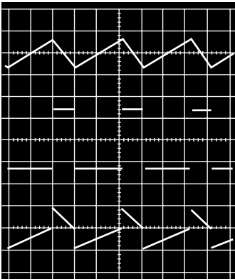
Figure 14 HA17741 Triangular Wave Generator Operating Waveform
