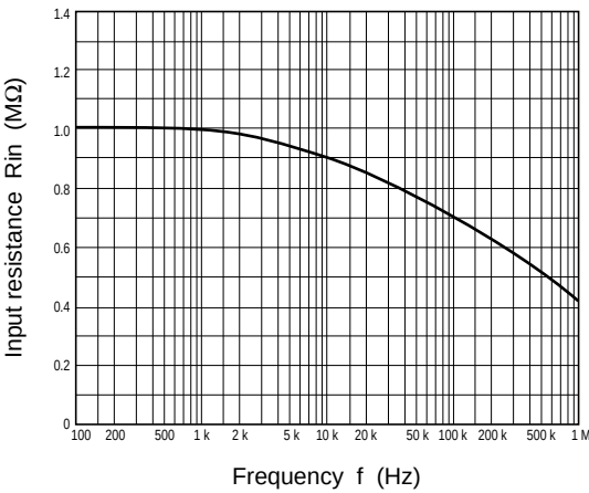
Input Resistance vs. Frequency Characteristics
