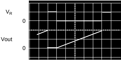
Figure 16 HA17741 Sawtooth Waveform Generator Operating Waveform
