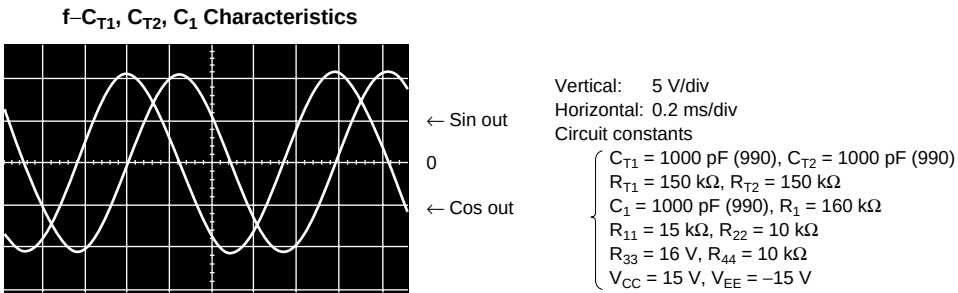
Figure 12 Sine and Cosine Output Waveforms
