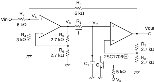
Figure 15 Sawtooth Waveform Generator
