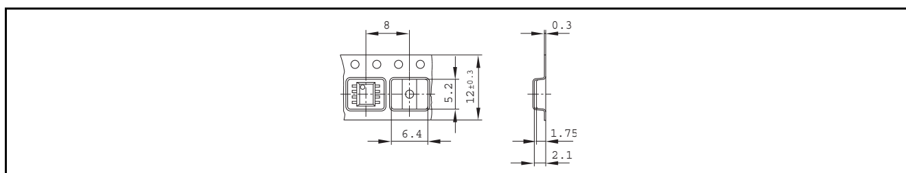
Figure 32 Tape and Reel
