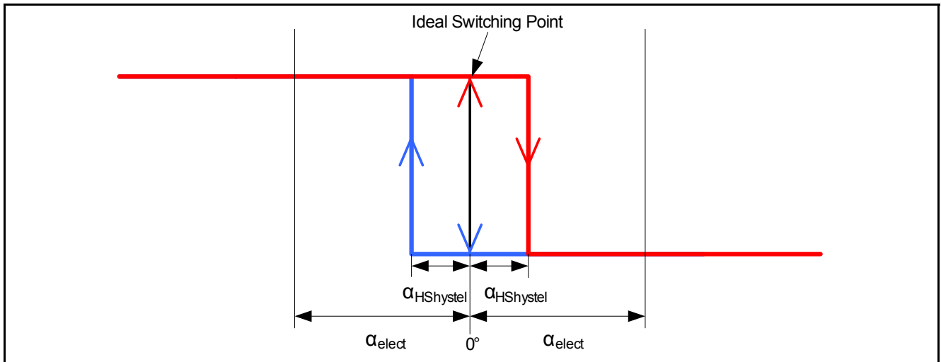
Figure 23 HS Hysteresis
