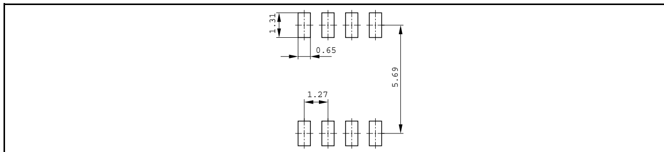
Figure 31 Footprint PG-DSO-8
