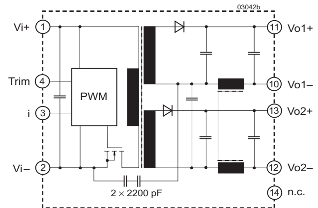
Fig. 2 Block diagram of dual-output models
