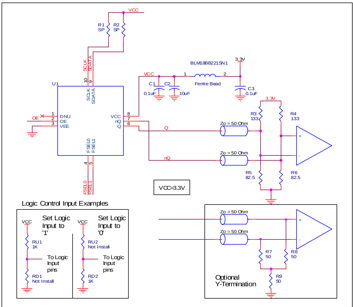
Figure 3. IDT8N3Q001 Application Schematic
