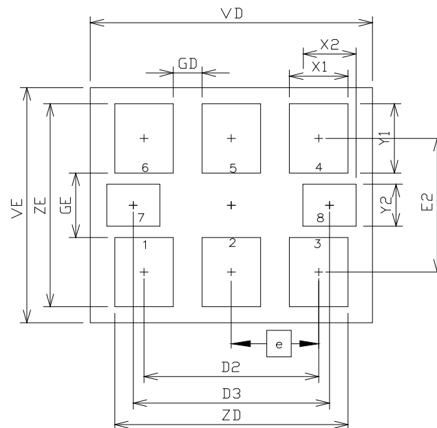
Figure 9. Si570/Si571 PCB Land Pattern
