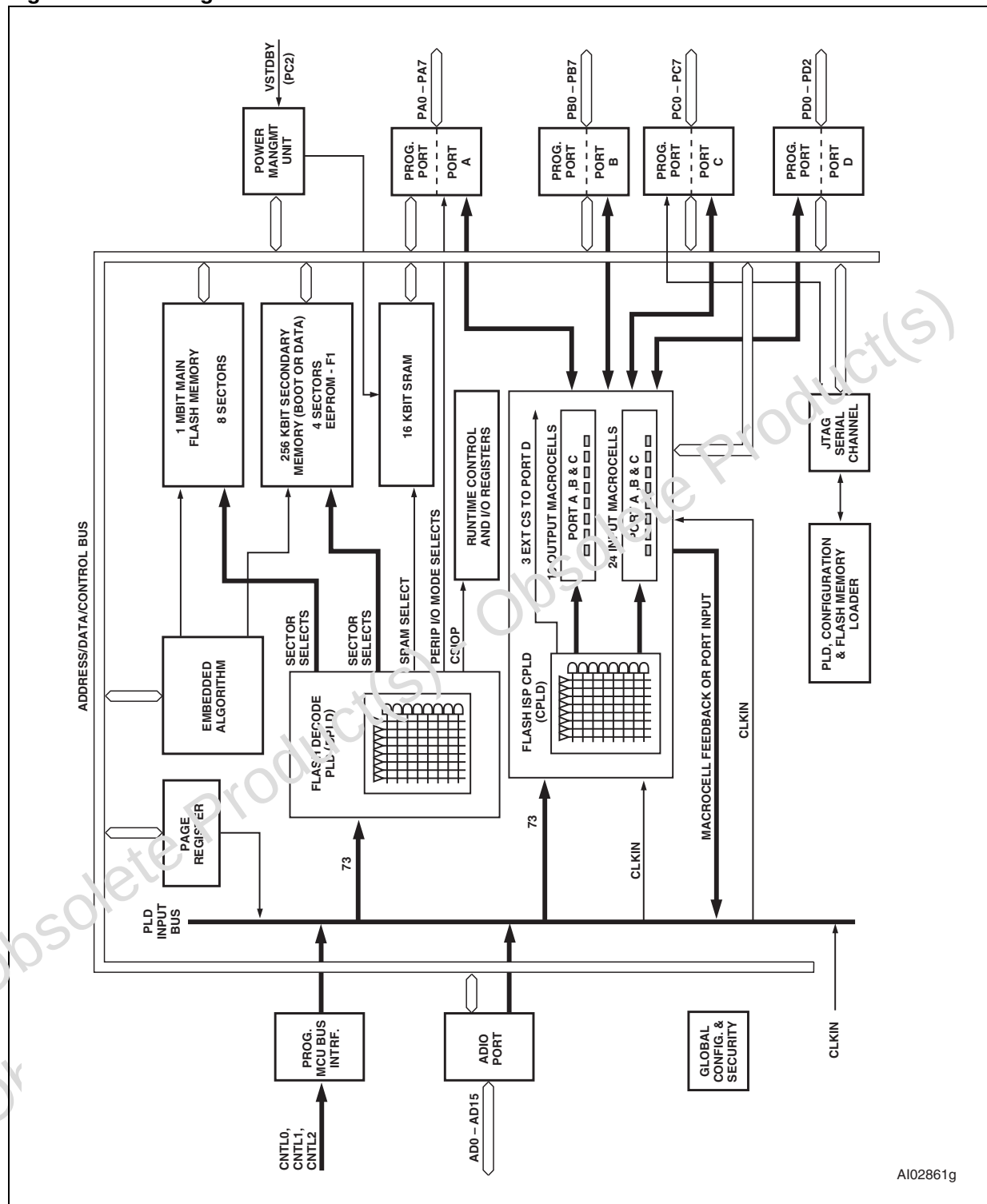
Figure 5. Block Diagram
