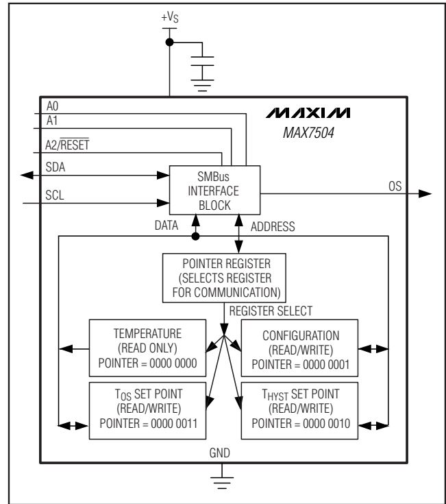
Figure 5. Block Diagram
