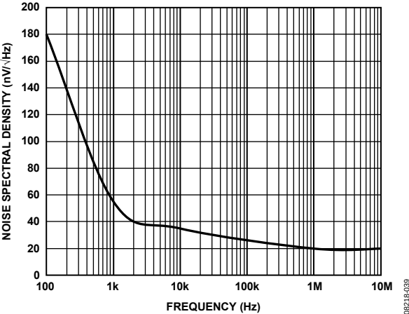
Figure 35. Noise Spectral Density of V_{OUT} , RF Input = -20 dBm, All C_{LPF} Values
