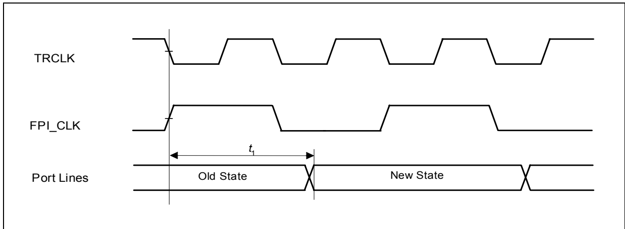
Figure 4-5 Port Timing
