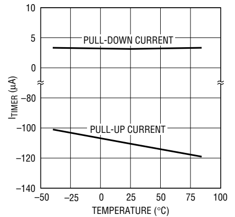
TIMER Pin Currents vs Temperature
