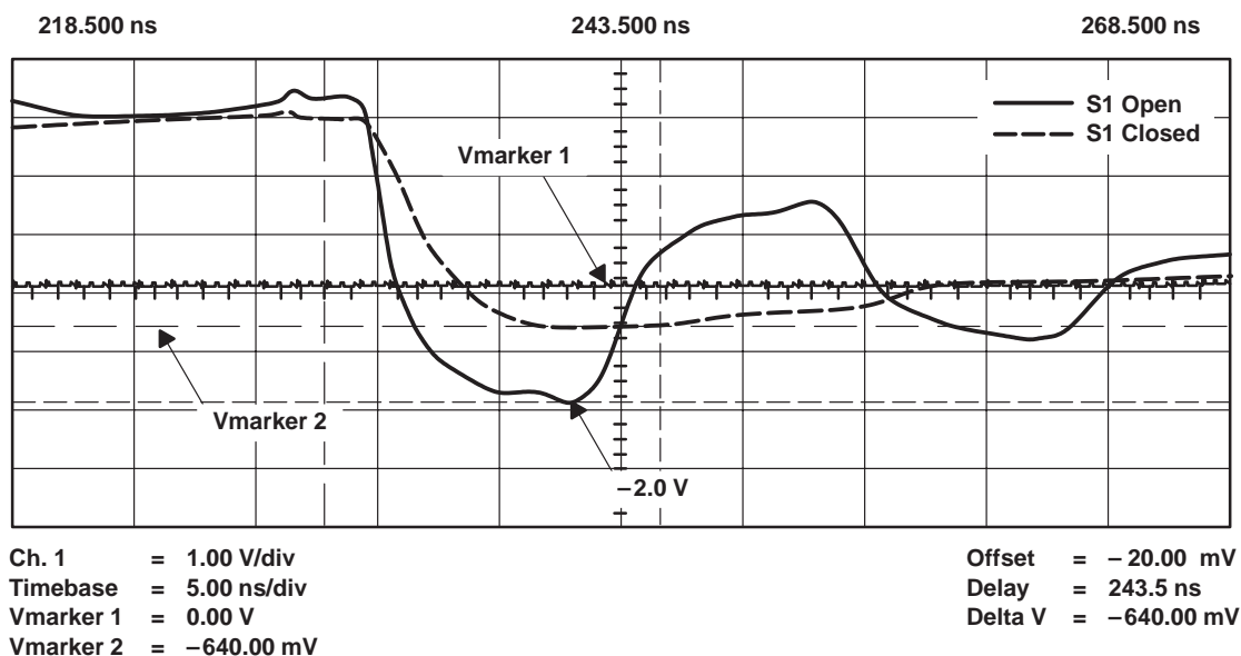
Figure 2. Undershoot Test Setup and Scope Display
