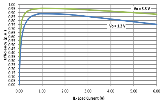
Efficiency vs Load Current, Vin = 5 V
