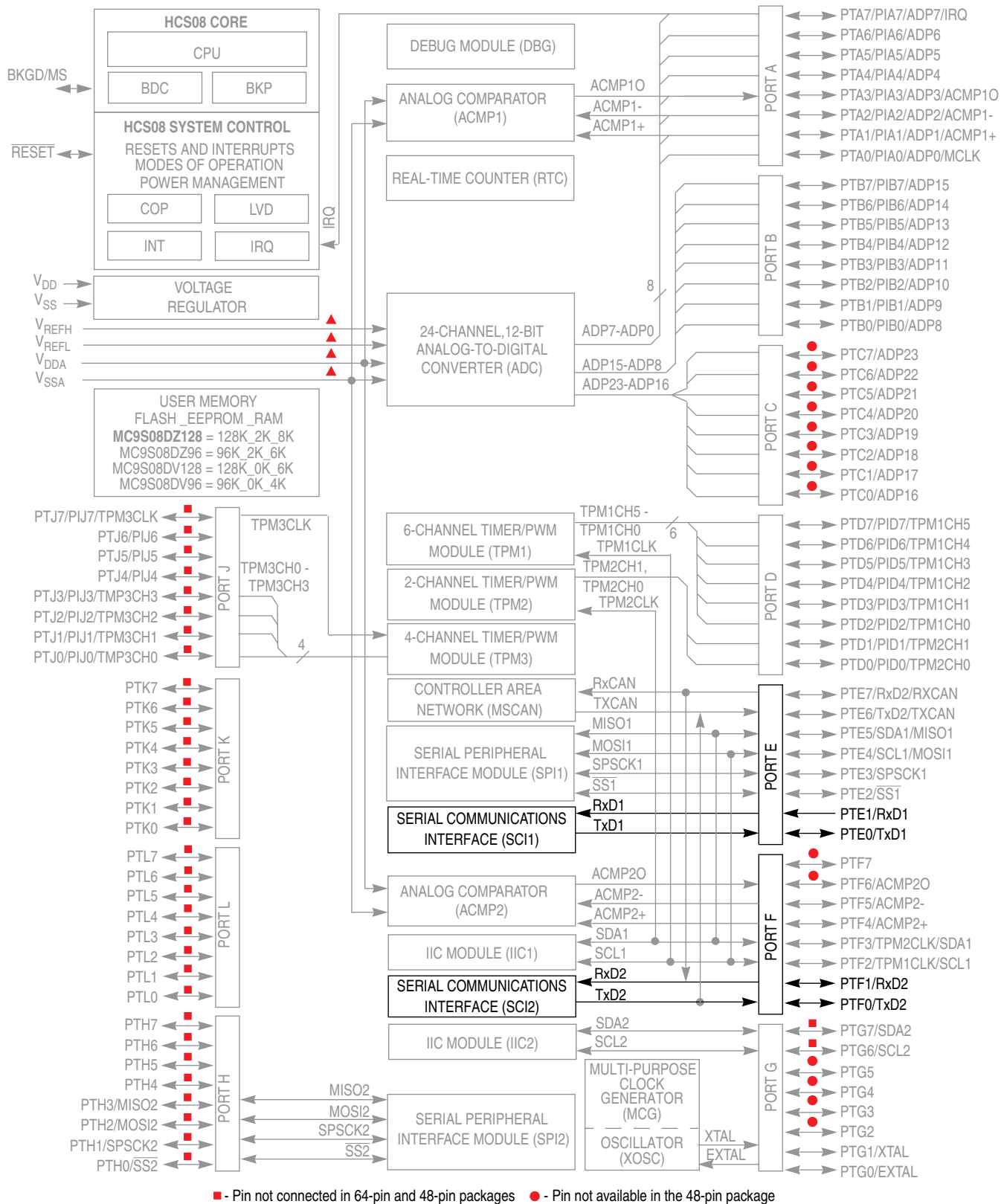
Figure 14-1. MC9S08DZ128 Block Diagram with SCI Highlighted
