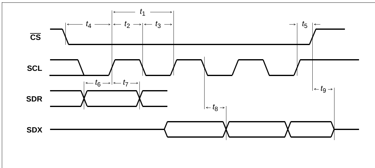
Figure 72 SCI Interface
