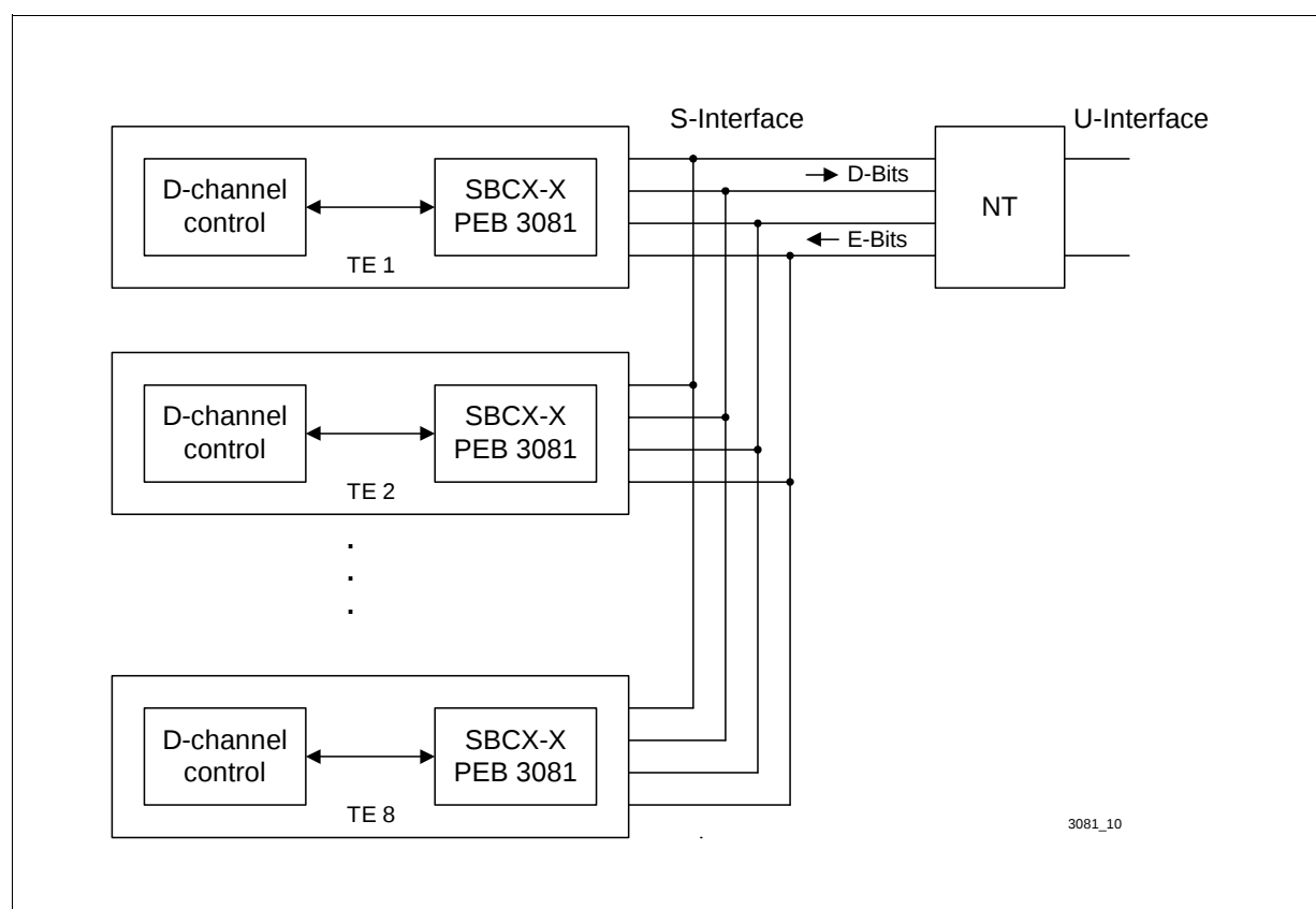
Figure 62 D-Channel Access Control on the S-Interface
