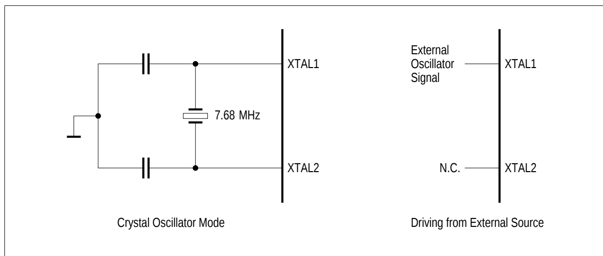
Figure 67 Oscillator Circuits
