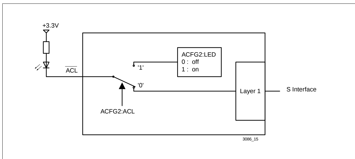
Figure 13 ACL Configuration
