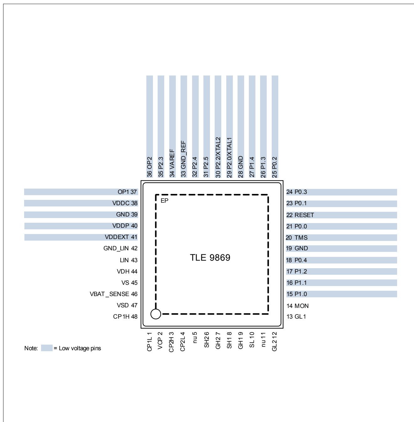
Figure 2 Device Pinout
