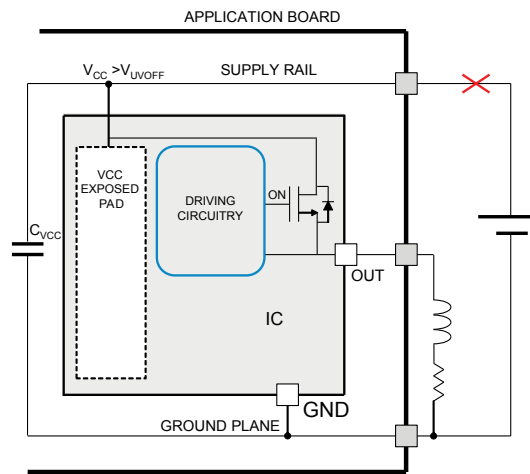
Figure 7. VCC disconnection
