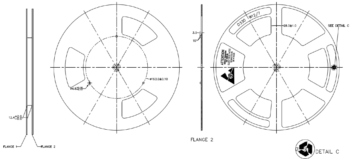
Figure 18. PowerSSO12 reel packing information [mm]
