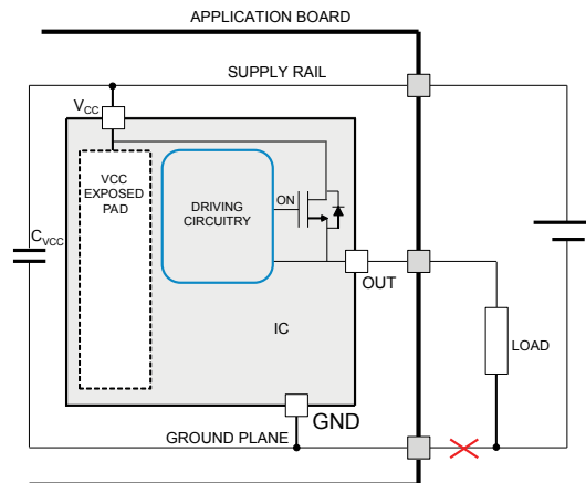
Figure 8. GND disconnection
