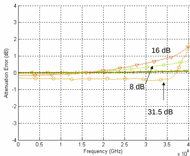
Figure 11. Attenuation Error Vs. Frequency
