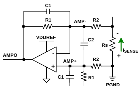
FIGURE 21. PRECISION CURRENT SENSE AMPLIFIER
