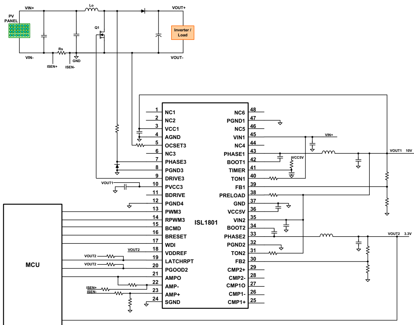
FIGURE 28. BOOST REGULATOR
