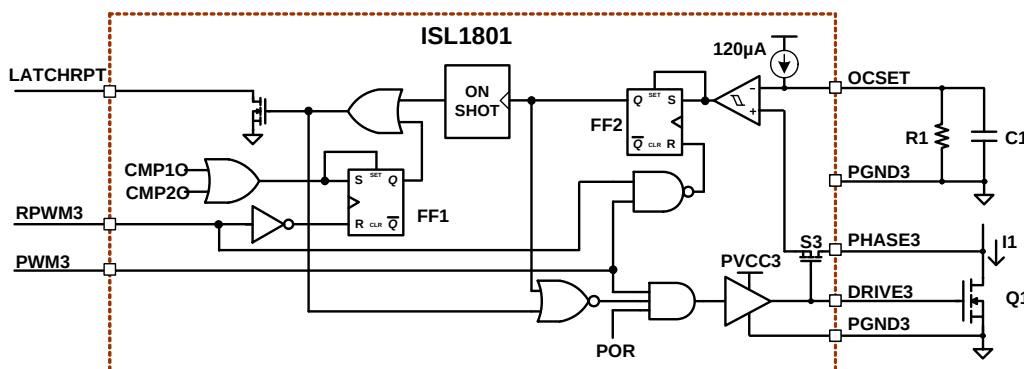
FIGURE 18. LOW-SIDE DRIVER LOGIC
