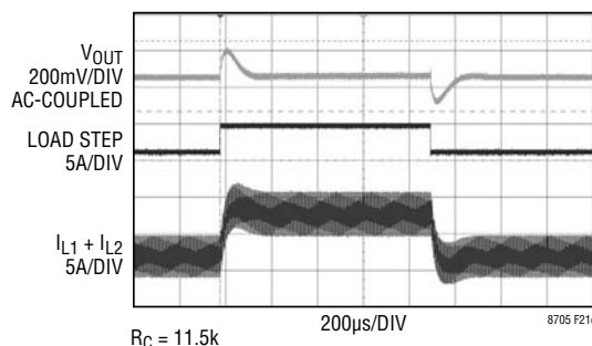
Figure 21c. Transient Response is Well Damped
