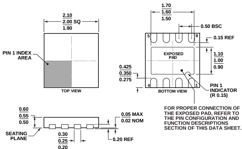
Figure 46. 8-Lead Lead Frame Chip Scale Package [LFCSF_UD] 2 mm x 2 mm Body, Ultra Thin, Dual Lead (CP-8-10)
