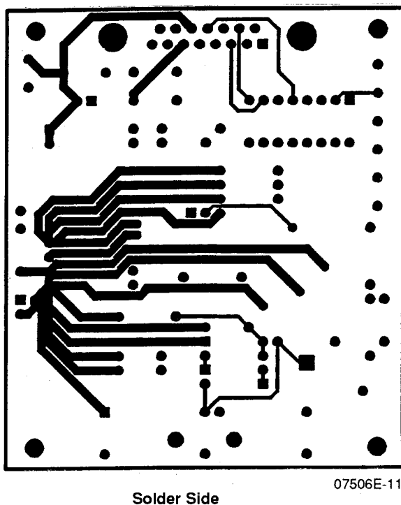
Figure 4-3. Suggested Printed Circuit Board Layout for a Four Layer PCB Application
