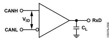
Figure 25. Receiver Voltage Measurements
