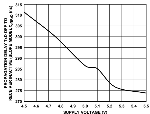
Figure 10. Propagation Delay (Slope Control Mode, R_{SLOPE} = 47\text{ k}\Omega ) from TxD Off to Receiver Inactive vs. Supply Voltage
