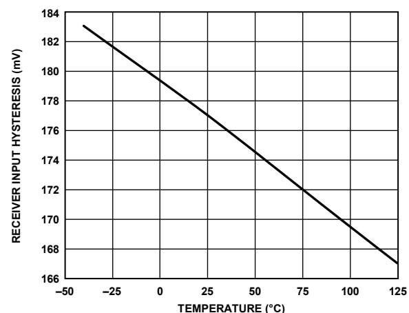
Figure 11. Receiver Input Hysteresis vs. Temperature
