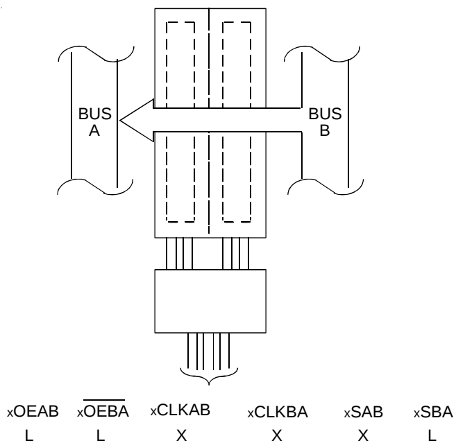
Real-time Transfer Bus B to A
