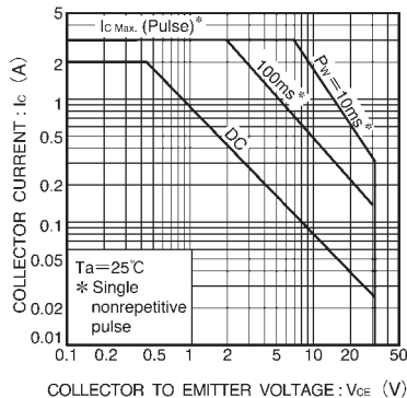
Fig.11 Safe operating area (2SD1055, 2SD1919)
