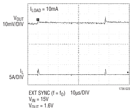
V_{OUT(RIPPLE)} (Synchronized)
