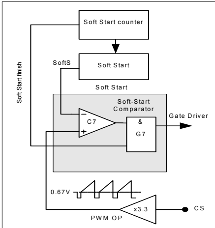
Figure 9 Soft Start
