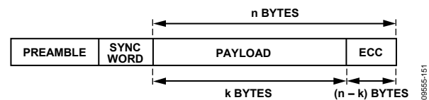
Figure 75. Packet Structure with Appended Reed-Solomon ECC
