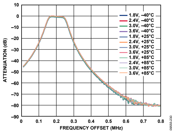
Figure 19. IF Filter Profile vs. V_{DD} and Temperature, 100 kHz IF Filter Bandwidth
